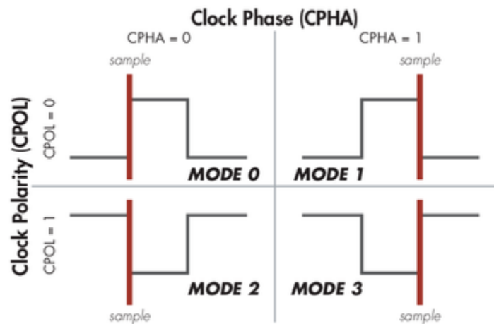
Figure 2 : SPI Modes
